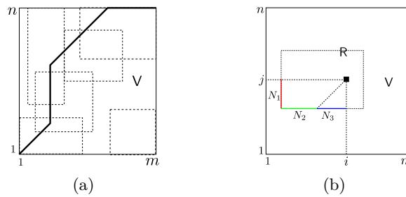
■ Figure 2. (a) Illustration of our algorithm: compute a small set of rectangles that covers the optimal admissible path from (1, 1) to (m, n) (drawn in bold); (b) partitioning the boundary points of rectangle R dominated by (i, j) .
