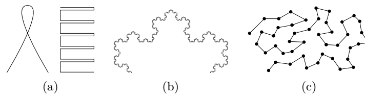
■ Figure 1. (a) \kappa -packed curves that are not \kappa -bounded. (b) The top half of the Koch snowflake is a \kappa -bounded curve that is not \kappa -packed. (c) A backbone sequence that is neither \kappa -bounded nor \kappa -packed.
